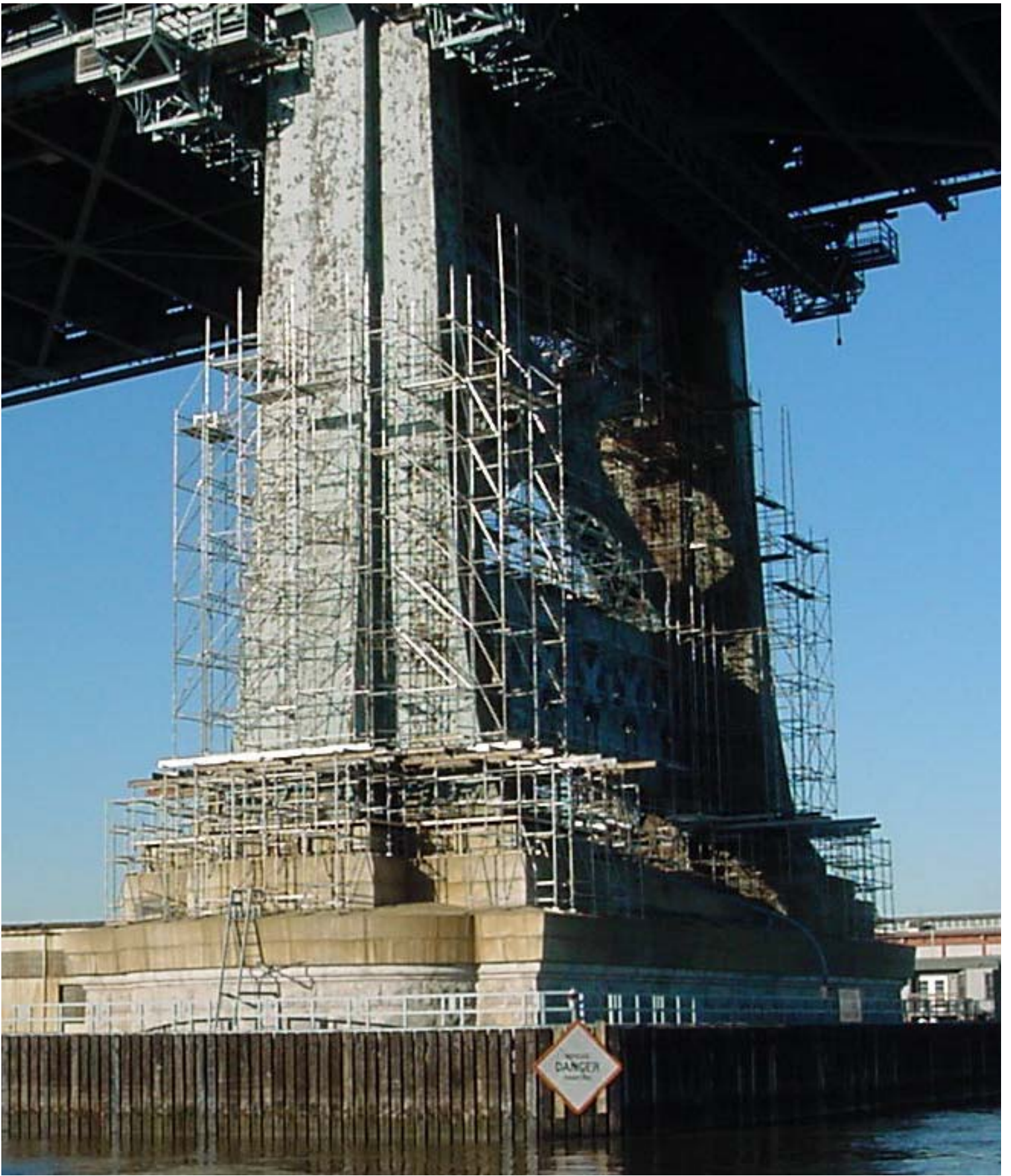
Scaffolding Installation Tower Base To Roadway
