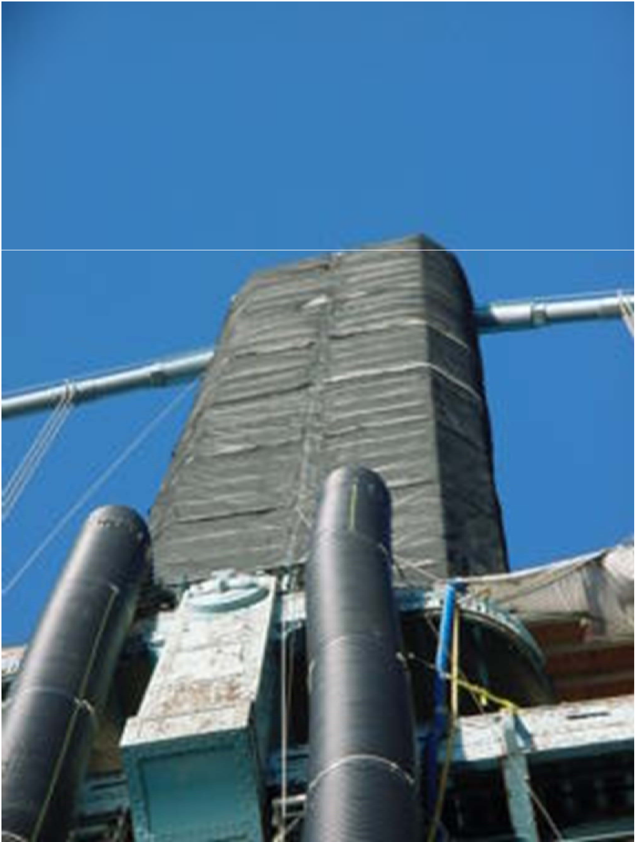
Containment Around Camden Tower
